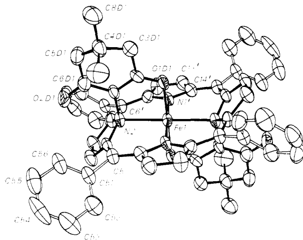
Figure 1. ORTEP plot of complex 2 . Hydrogen atoms are omitted for clarity. Ellipsoids are scaled to enclose 40% of the electronic density.
